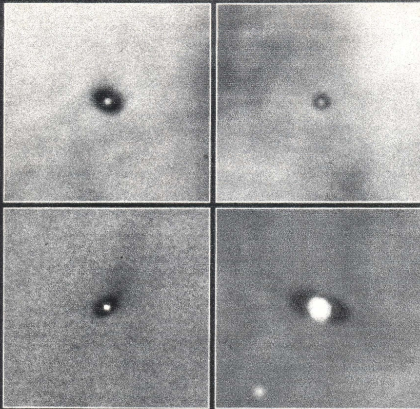
Protoplanetary Disks · Orion Nebula Hubble Space Telescope · WFPC2
